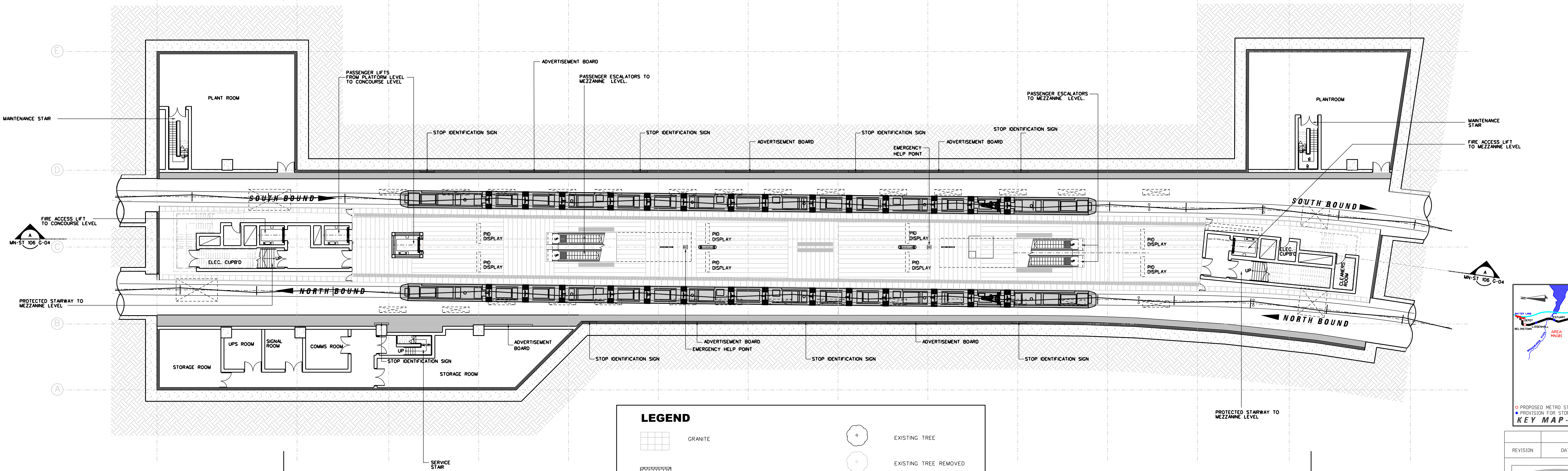
PLATFORM LEVEL PLAN SCALE 1:200
