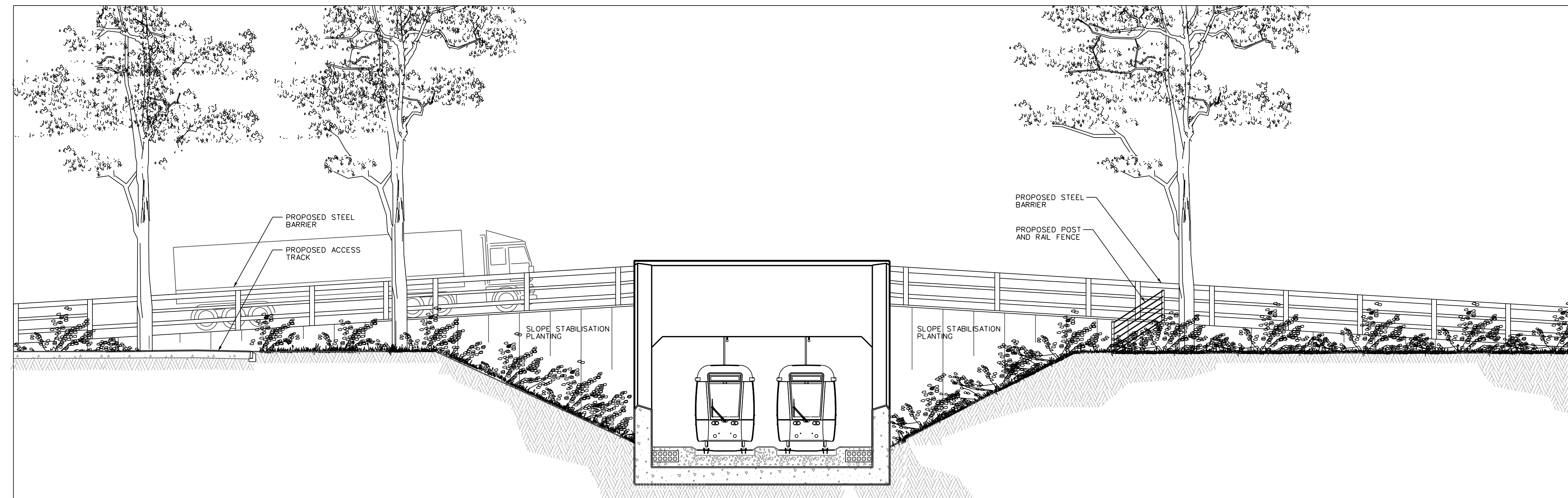
SECTIONAL ELEVATION A-A SCALE 1:100
