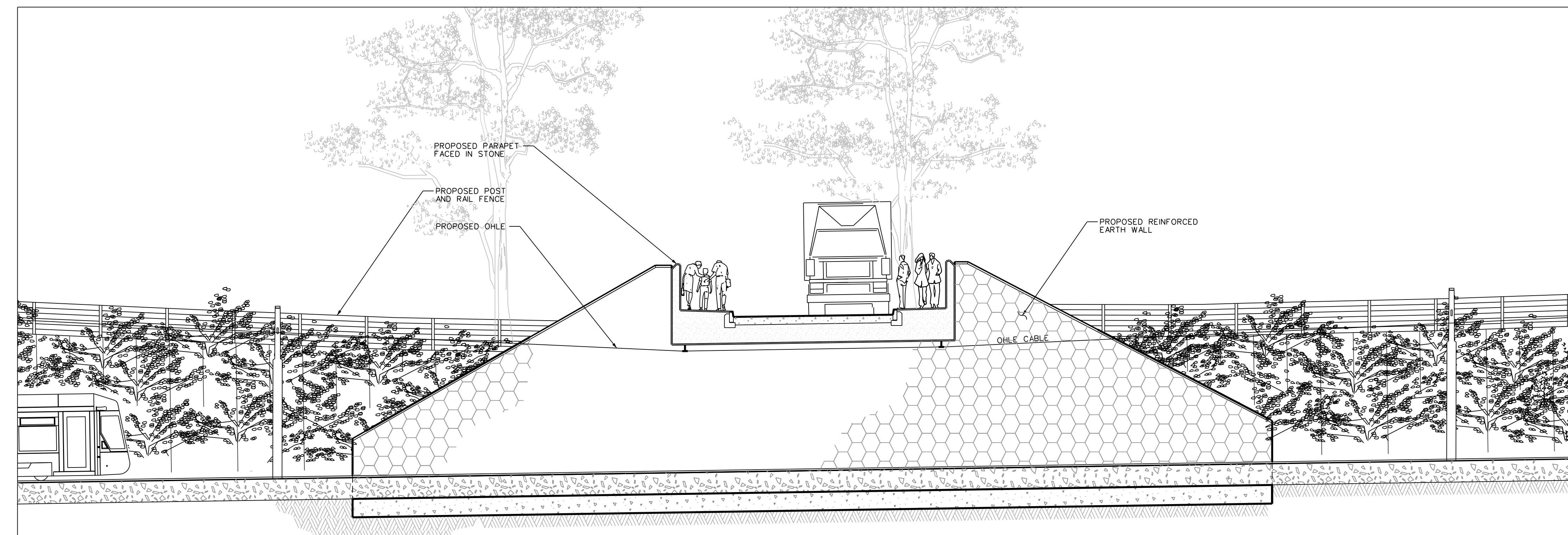
SECTIONAL ELEVATION B-B SCALE 1:100
