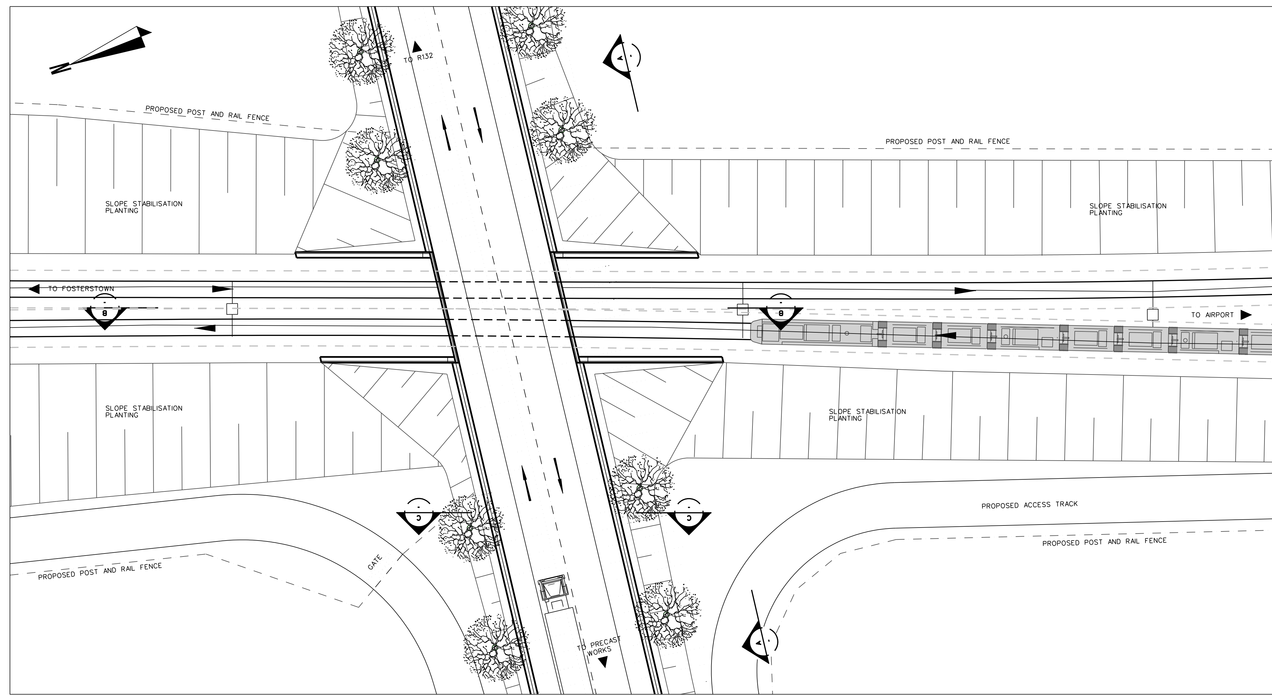
PLAN 1:200 SCALE 1:200
