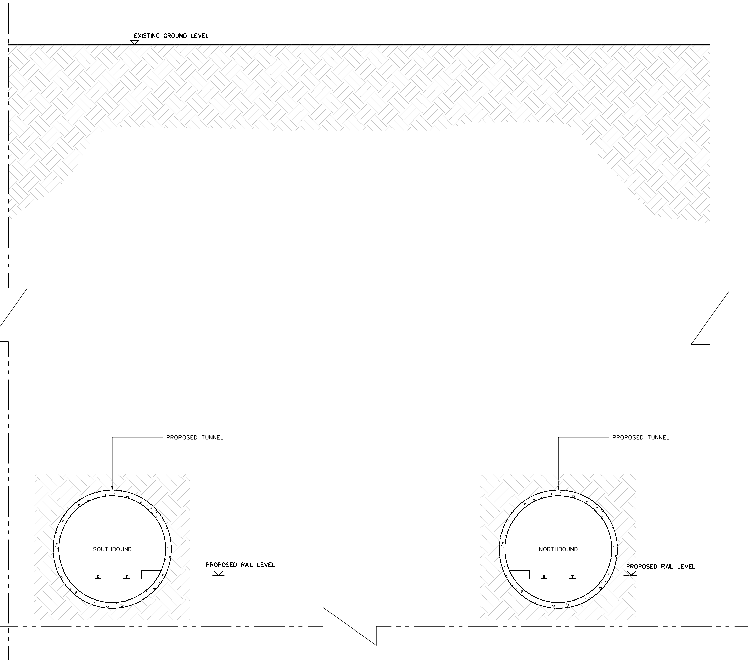
CROSS SECTION 07-02 SCALE 1:100
